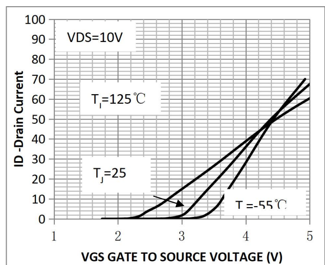
Figure.12 Transfer Characteristics
